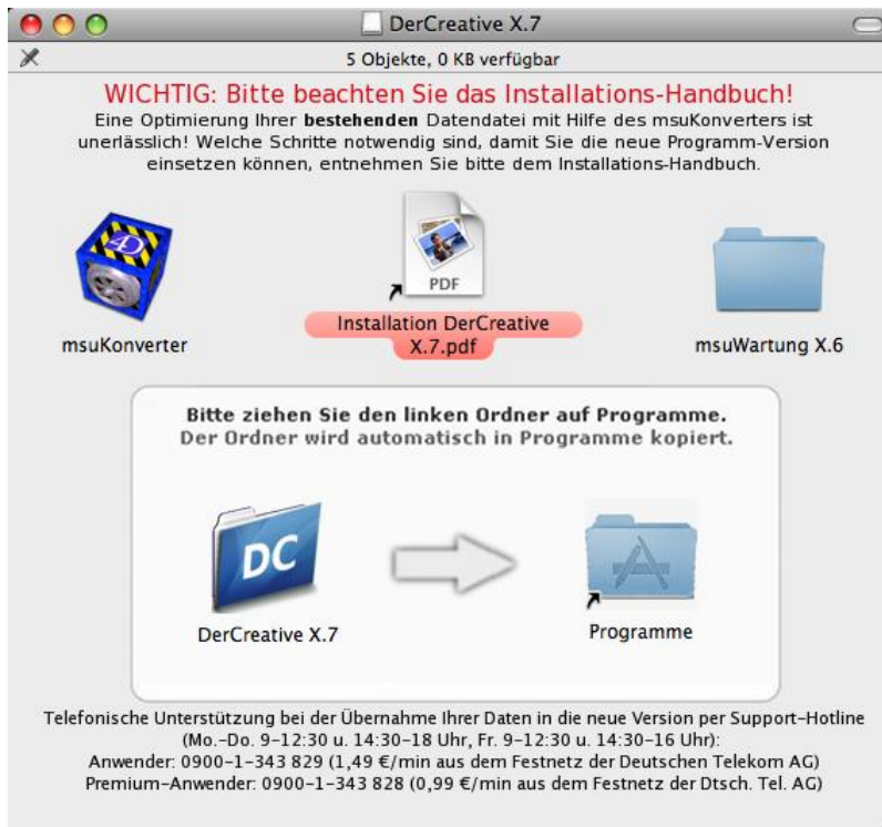
Installations-Fenster
